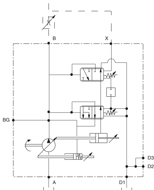
Load Sensing and Pressure Limiter Control with Optional Minimum & Maximum Displacement Adjustments (A minimum displacement stop requires the use of a system relief valve.)
