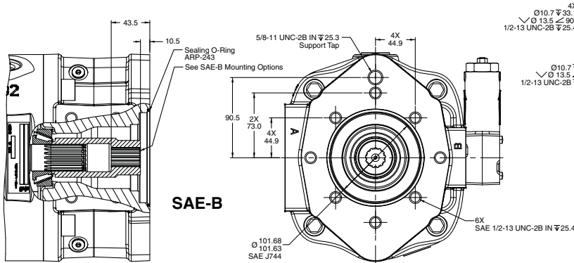
SAE 22-4 (B) (T0*B) & SAE 25-4 (B-B) (T0*Q) 4 BOLT & VERTICAL OR HORIZONTAL 2 BOLT
