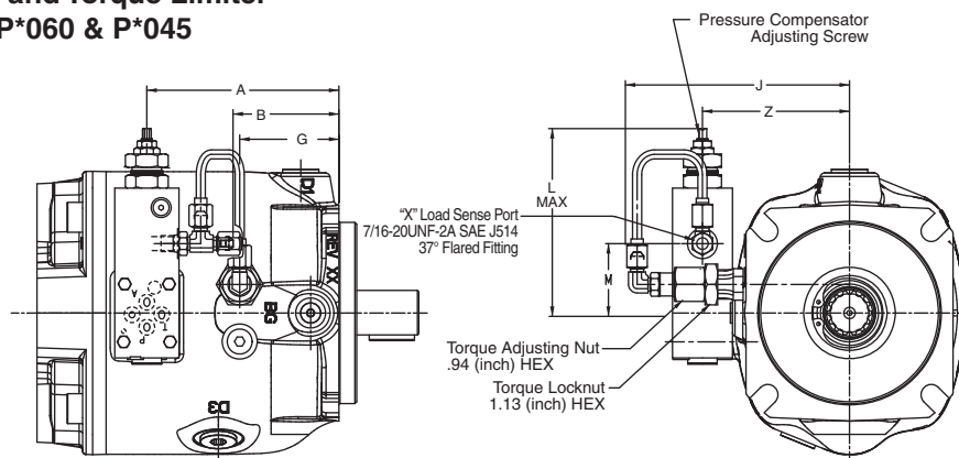
CW ORIENTATION P*060 SHOWN
