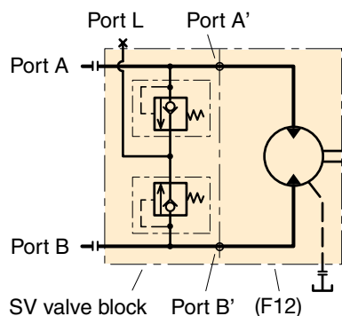
Hydraulic schematic.
